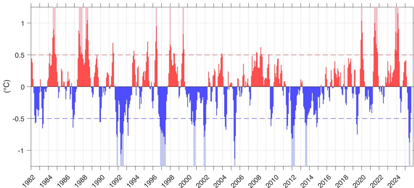
Figure 2. Monthly sea surface temperature anomalies in the eastern equatorial Atlantic ( 20^{\circ}\text{W}-0^{\circ} , 3^{\circ}\text{S}-3^{\circ}\text{N} ; ATL3 region) from January 1982 to September 2025 from satellite observations. Blue bars indicate cold anomalies, red bars warm anomalies. Each value represents a mean of 3 consecutive months. Only if three consecutive mean values exceed the \pm 0.5^{\circ}\text{C} threshold (red and blue dashed lines) it is called warm or cold event. Such warm and cold events are marked by red and blue shadings, respectively. The long-term warming trend of 0.75^{\circ}\text{C} between 1982 to 2025 has been removed from the time series.
