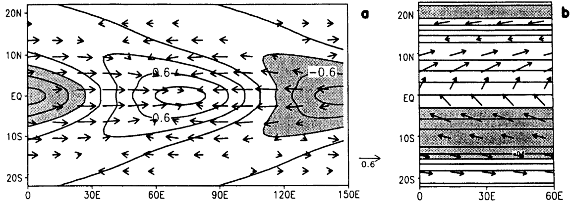
Figure 9: Dominant modes at a , the Pacific and b , the Atlantic wavelengths in the coupled model. SST in contours ( < -0.3^{\circ}\text{C} shaded) and surface wind velocity (m/s) in vectors.
