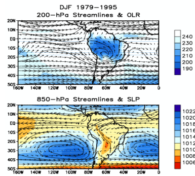
Figure 2. Mean (1979-1995) 200-hPa vector wind/ streamlines and outgoing longwave radiation (OLR) (top) and 850-hPa vector wind/ streamlines and sea level pressure (SLP) (bottom). Units are \text{W m}^{-2} for OLR and hPa for SLP. Circulation data are derived from the NCEP/ NCAR CDAS-Reanalysis data archive.
