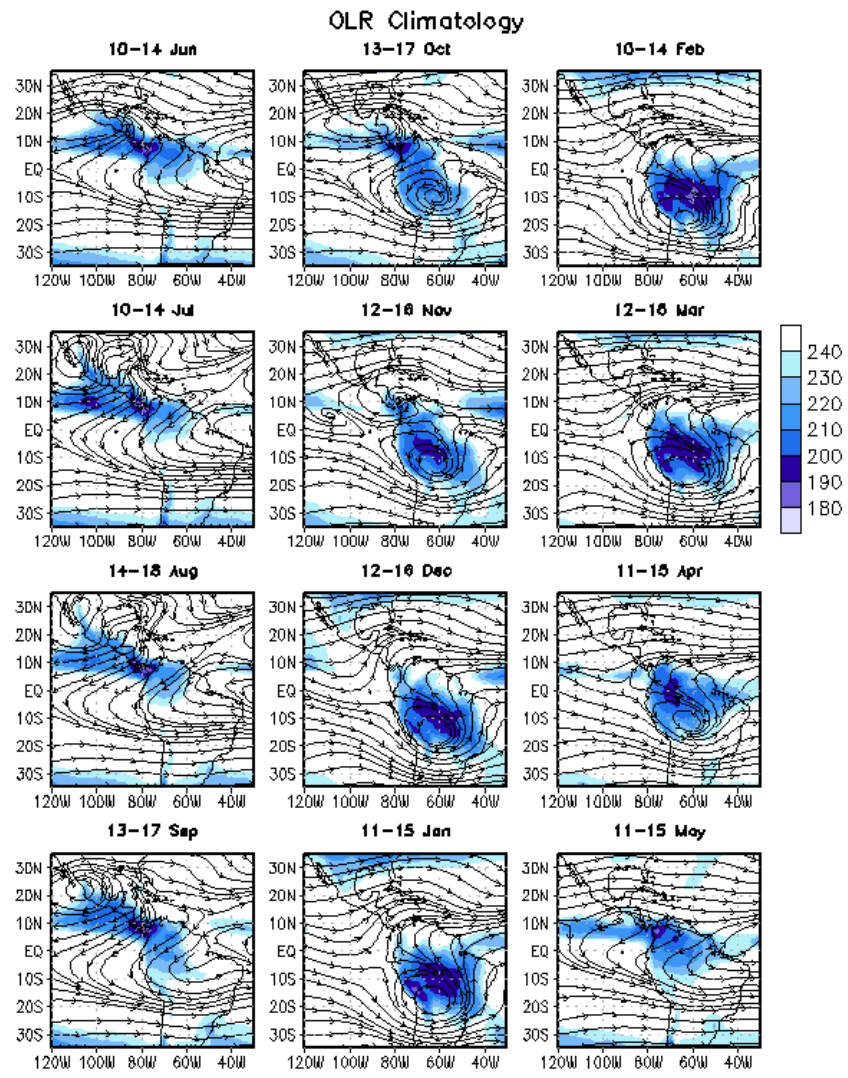
Figure 4. Mean (1979-1995) seasonal cycle of OLR and 200-hPa streamlines. Units for OLR are \text{W m}^{-2} . Low values of OLR indicate cold cloud tops (deep convection) in the Tropics.
