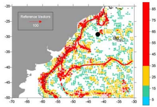
Figure 2: Surface current velocity field derived from 10 years of surface drifter observations. The black dot indicates the location of the proposed observing site.
