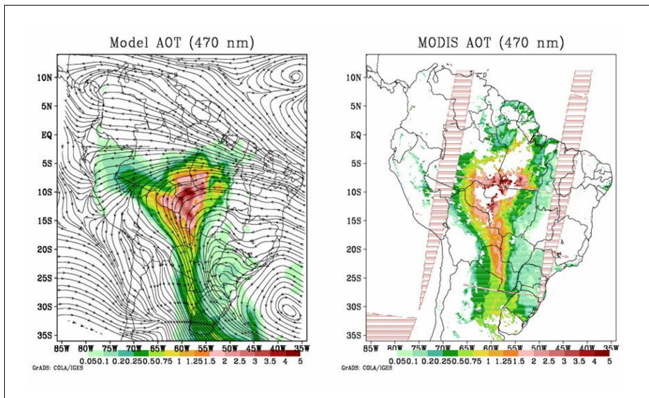
Figure 6.3 Numerical simulation and validation with MODIS of aerosol optical thickness. Freitas et al (2005)
