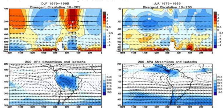
Figure 3. Vertical-longitude cross-section of the mean (1979-1995) divergent circulation (vectors) for the latitude band 10^{\circ} - 20^{\circ} S (top panels) and mean (1979-1995) 200-hPa vector wind/ streamlines and OLR (bottom panels) for December-February (left panels) and June-August (right panels). Units are 10^{-6} \text{ s}^{-1} for divergence (contours and shading in top panels) and \text{W m}^{-2} for OLR (shading in bottom panels).
