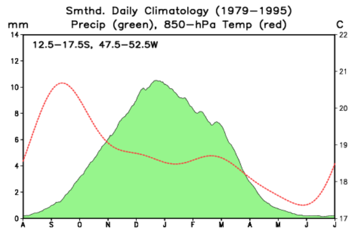
Figure 5. Mean (1979-1995) daily precipitation (mm) for central Brazil (12.5°-17.5°S, 47.5°-52.5°W) (shaded in green), 850-hPa temperature (degrees C, red curve, top panel), and 850-hPa zonal wind ( \text{mm s}^{-1} , red curve, bottom panel).
