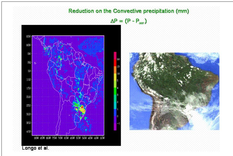
Figure 6.4. The figure on the left shows the difference in convective precipitation between two experiments without and with the aerosol-radiation interaction for the situation on the right, showing the corresponding satellite images. Red colors (positive values) indicated reduction in accumulated precipitation.
