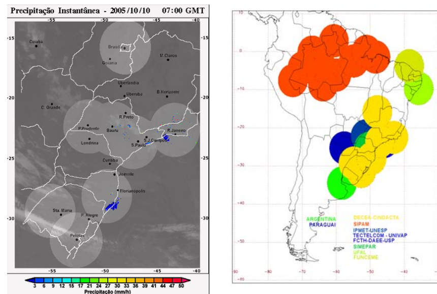
Figure 6.6. On the left the meteorological radar coverage in Southern Brazil. On the right the same for So. America.
